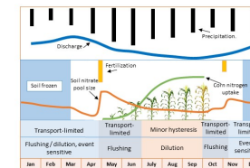
Fig. 7 Conceptual model for fate, transport and pathways of nitrate in different seasons.
