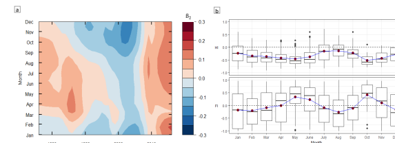
Fig. 6 Long-term seasonality of C-Q relationship from WRTDS (a) and storm hysteresis metrics (b).
